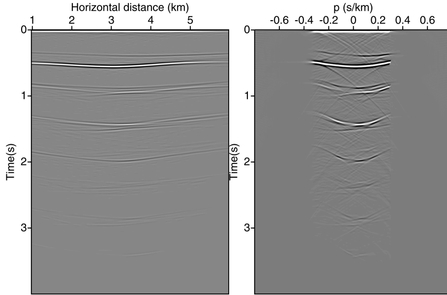
Figure 4. The crosscorrelogram for a master trace recorded at (3km,0) with a slave trace recorded at the same location for each subsurface position (only positive time is shown). Left: with time-space domain interferometry. Right: with plane-wave domain interferometry.
