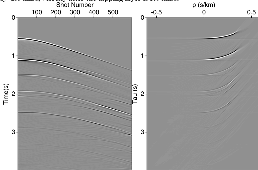
Figure 3. Common receiver gather for the first receiver (left) and its tau-p transformed gather (right). There are 200 ray parameters in the plane-wave gather from -0.6 to 0.6 s/km.
