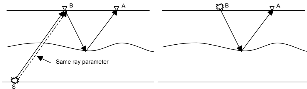
Figure 1. Crosscorrelating traces recorded at receiver locations B and A produces a new trace with virtual source at B, receiver at A. The canceled overlapping raypaths in the plane-wave domain corresponds to same ray parameters.
